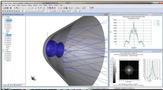
Figure 2: Side Emitting LED with lens and reflector combination.
